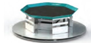
NPP/L-45 — a 450 mm diameter two-level turntable platform with an upper tray, it can be additionally equipped with 4 Cocis A type bins and 4 Cocis B type bins. Height - 109 mm
